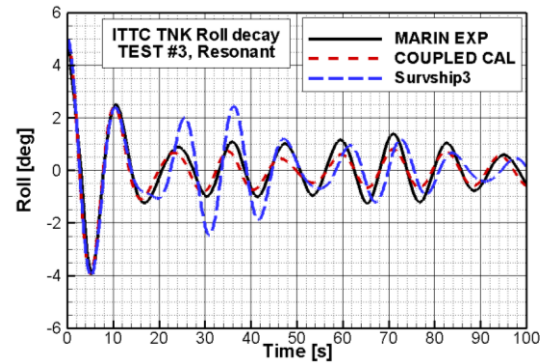
Fig 19: Free decay-resonance ( h=4 m)
