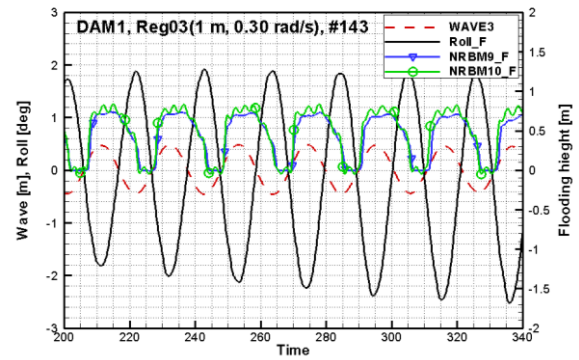
Fig 12: Motion and flooding of DAM1 (wave height 1m, \omega=0.3 rad/s)
