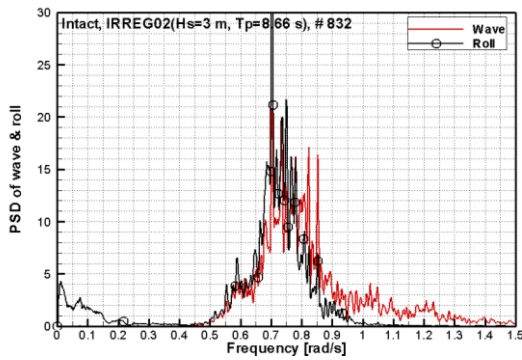
Fig 15: PSD of intact in irregular wave ( H_s=3 m)
